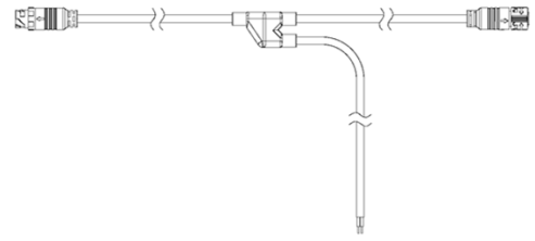
Y-connector kit 5P DC/DMX
